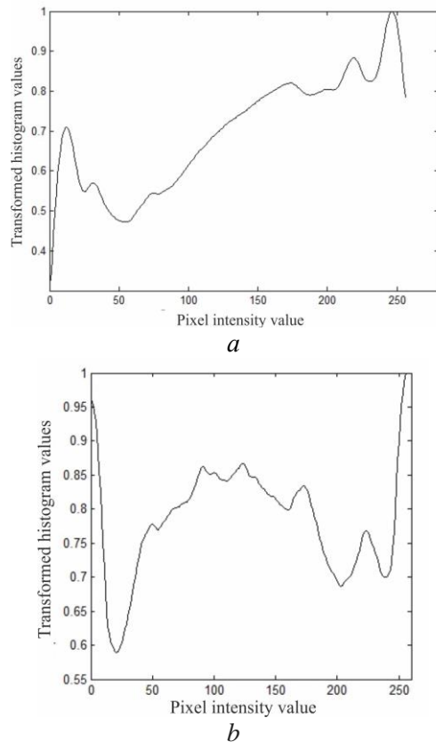
Fig. 3. Transformed image histogram after image linear filtering: a – in rows; b – in columns Source: compiled by the author
