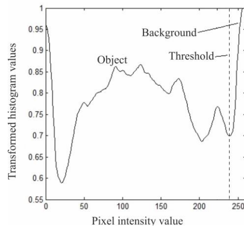
Fig. 4. Threshold selecting for extracting text regions Source: compiled by the author
