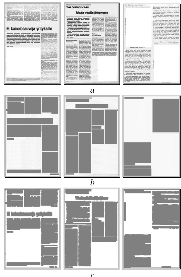
Fig. 6. The results of the text regions extraction on scanned document images: a – original images; b – ground-truth segmentation results; c – the results of the text regions extraction
