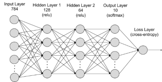
Fig. 3. Architecture of multilayer perceptron
