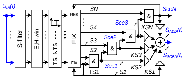
Fig. 7. Block diagram of the S-detector SceN . Recognition of the top hierarchical level of dynamic pattern recognition
