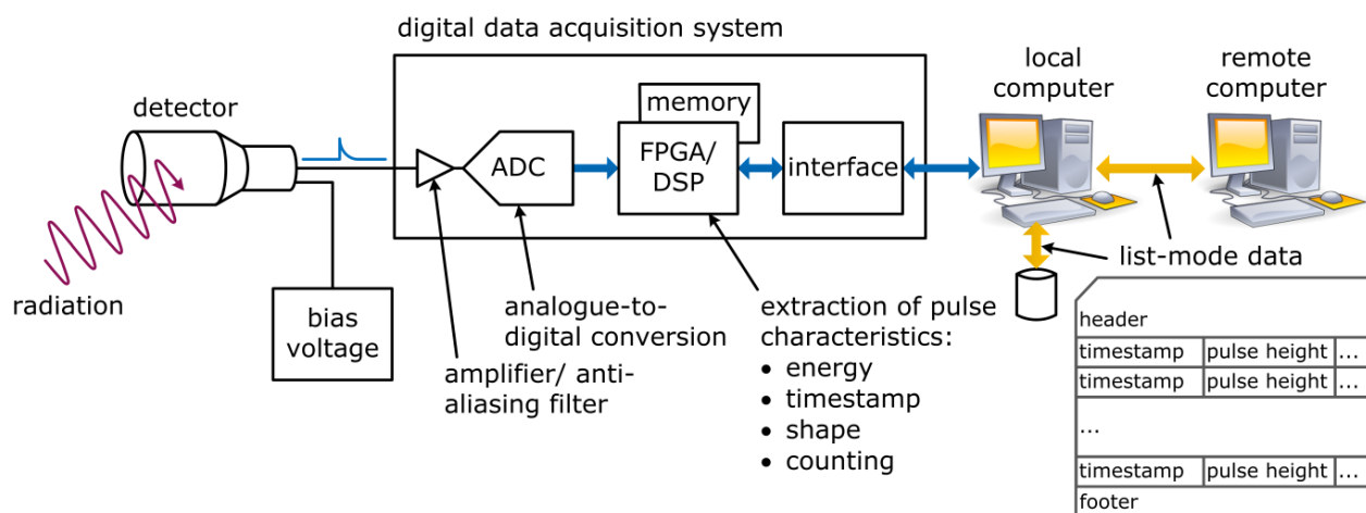
Fig. 1. Typical data acquisition scheme used with modern radiation detectors [3]
