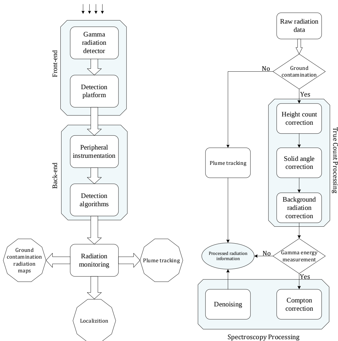
Fig. 2. Radiation monitoring system [12]
