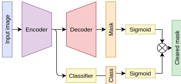
Fig. 6. Inference neural network graph
