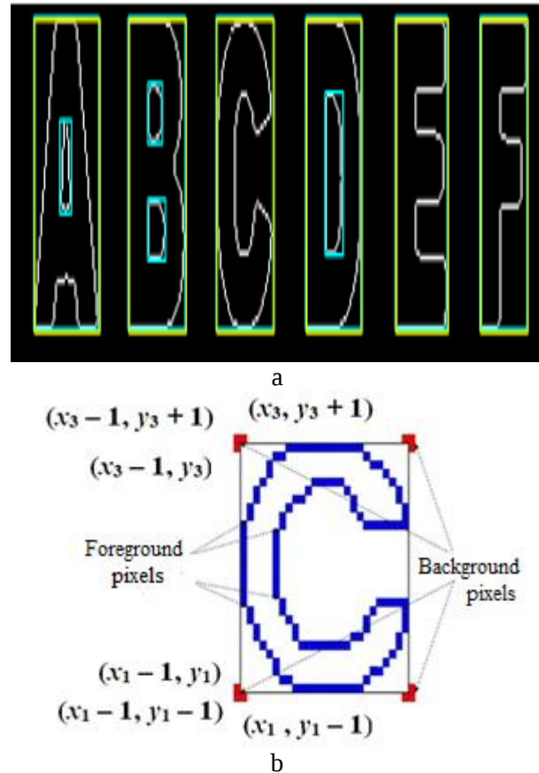
Fig. 1. Rectangles, described around text characters:
