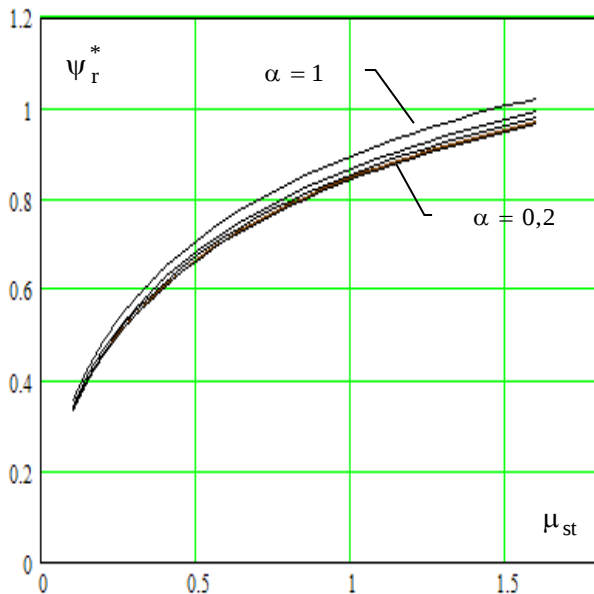
Fig. 3. Dependences of extreme values \Psi_r for Q_s from the moment of loading \mu_{st} = M_{st}/M_n at different speeds
