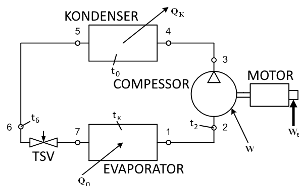
Fig. 2. SRU structural scheme
