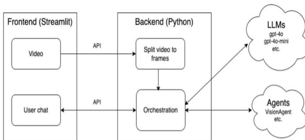
Fig. 2. Program structure
