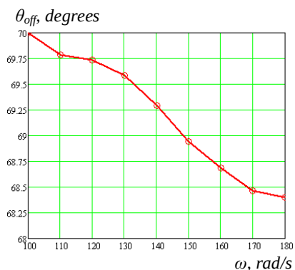
Fig. 13. The relationship between the angle of turning off the corresponding phases of the switched reluctance motor and the speed of rotation of its shaft
