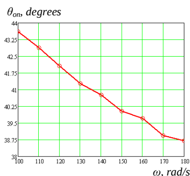
Fig. 12. The relationship between the angle of turning on the corresponding phases of the switched reluctance motor and the speed of rotation of its shaft
