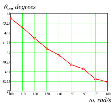
Fig. 12. The relationship between the angle of turning on the corresponding phases of the switched reluctance motor and the speed of rotation of its shaft
