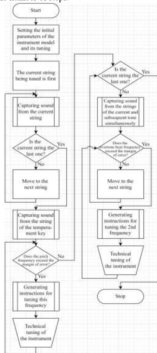
Fig. 4. Block diagram of the proposed method of automated professional tuning of acoustic string musical instruments
