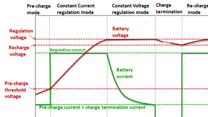
Fig. 2. Change in current and voltage when charging a lithium-ion battery according to the constant current / constant voltage rule
