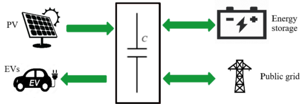
Fig. 1. Direct current micro grid for electric vehicle charging station
