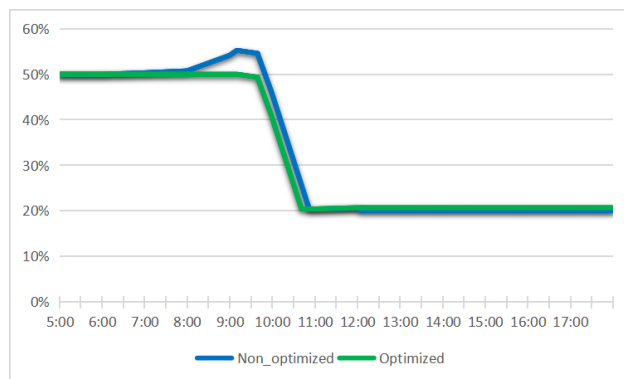
Fig. 13. Comparison of state-of-charge for modes with and without optimization in winter
