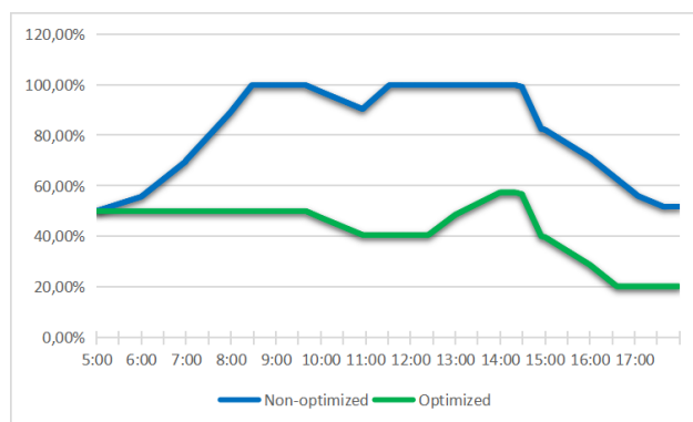
Fig. 8. Comparison of state-of-charge for modes with and without optimization in summer
