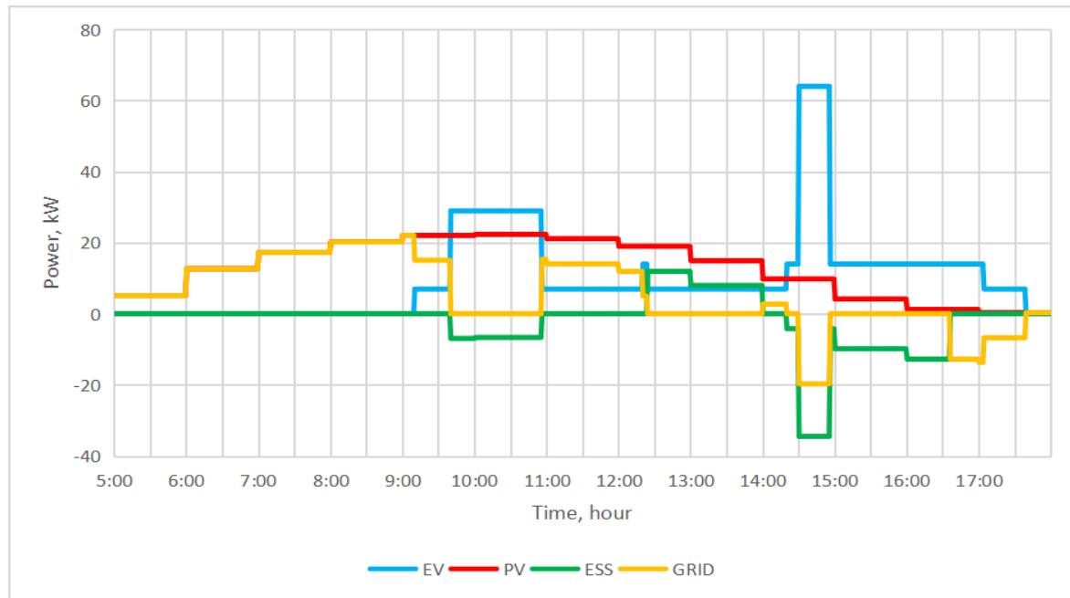
Fig. 7. Power dispatch in operating mode with optimization (summer)
