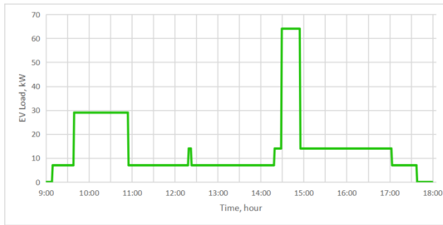
Fig. 4. Estimated car load schedule
