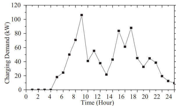
Fig. 3. Expected charging demand of a fast charging station on a weekday Source: compiled by the [20]
