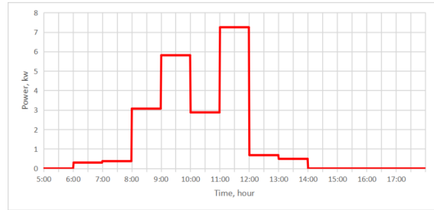
Fig. 10. Graph of electricity generation by photovoltaic module in winter
