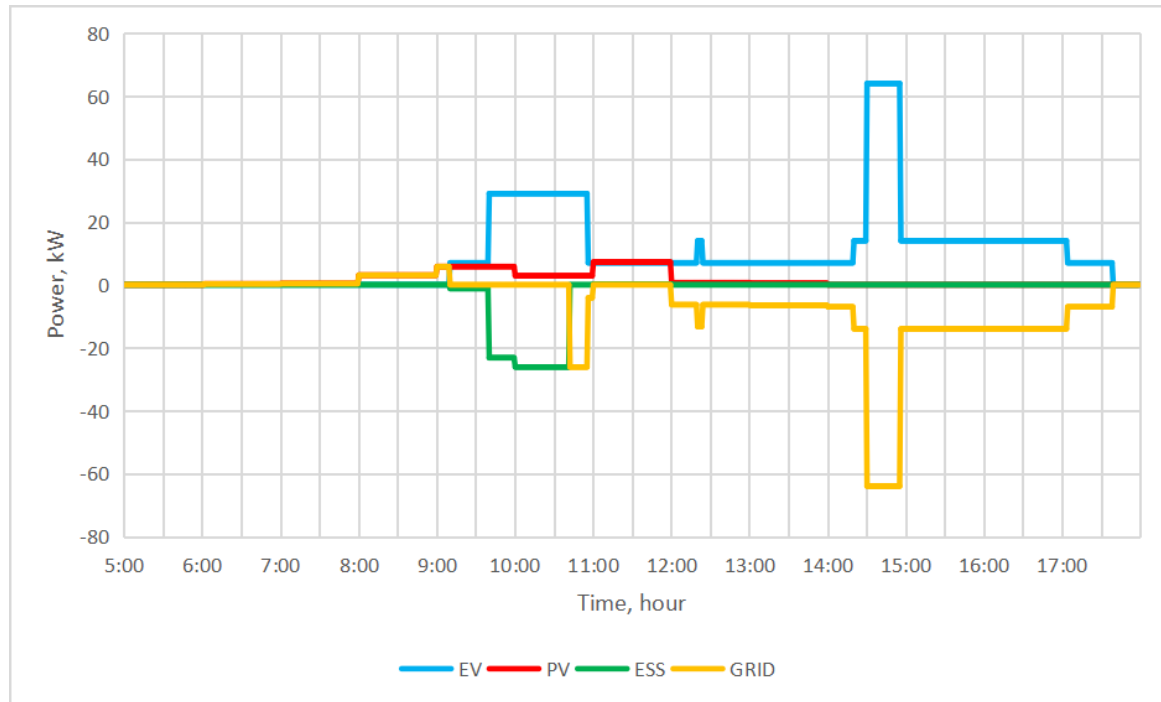
Fig. 12. Power dispatch in operating mode with optimization (winter)
