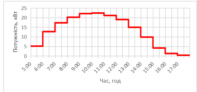
Fig. 5. Graph of electricity generation by photovoltaic module in summer
