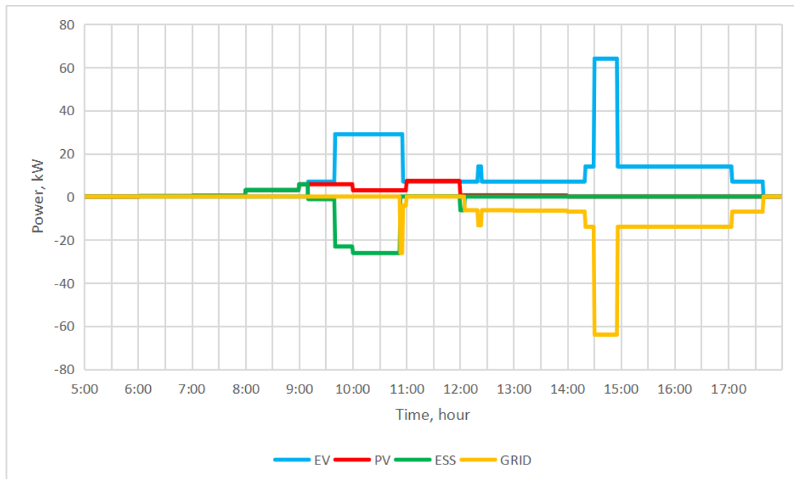
Fig. 11. Power dispatch in operating mode without optimization (winter)
