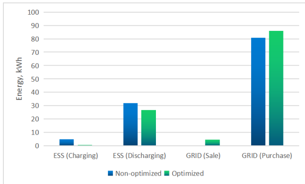
Fig. 14. Comparison of energy dispatch for modes with and without optimization in winter Source: compiled by the authors
