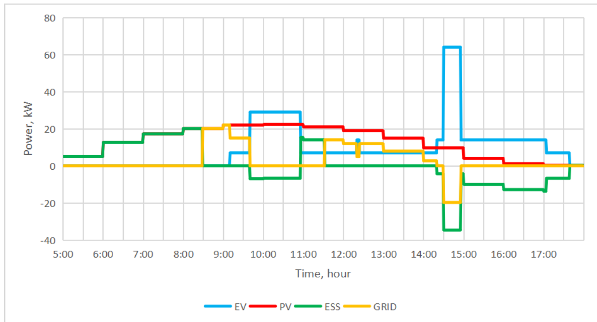
Fig. 6. Power dispatch in operating mode without optimization (summer)
