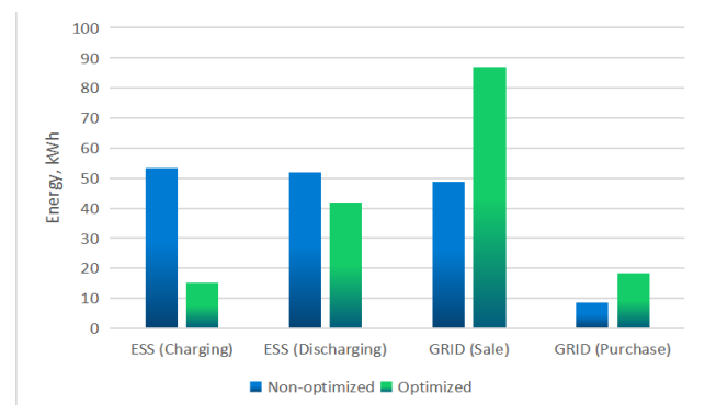
Fig. 9. Comparison of energy dispatch for modes with and without optimization in summer
