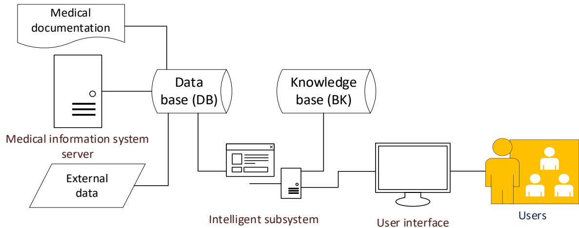
Fig.1. Architecture of an intelligent information system for forecasting components of medical projects
