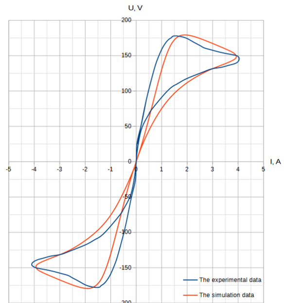
Fig. 13. The dynamic current–voltage characteristic of the arc for f = 50 Hz Source: compiled by the authors
