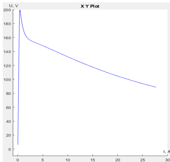
Fig. 15. The dynamic voltage-ampere characteristic of the electric arc under direct current
