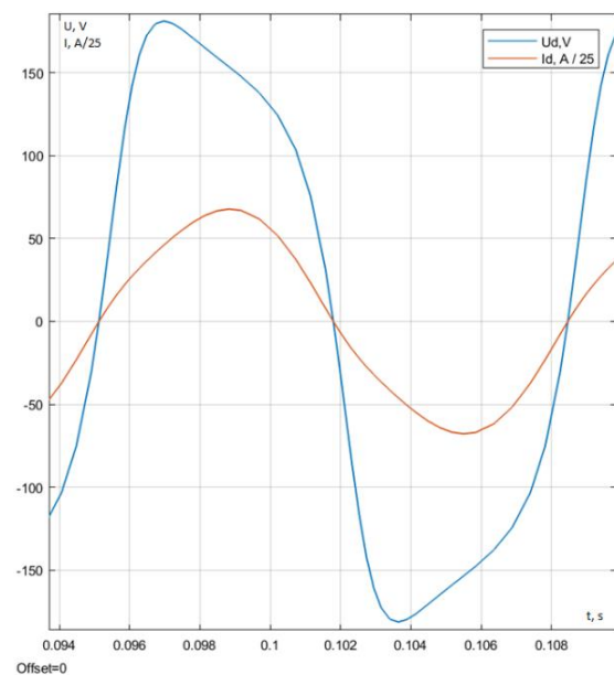
Fig. 20. The dependency of voltage u_d and current i_d of the electric arc on time, f = 75 Hz Source: compiled by the authors
