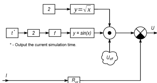
Fig. 8. The visual model of the alternating current voltage power source
