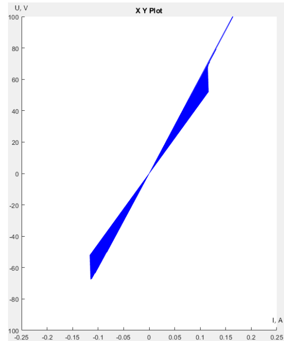
Fig. 27. The dynamic voltage-ampere characteristic (VAC) for the electric arc, f = 2.5 kHz
