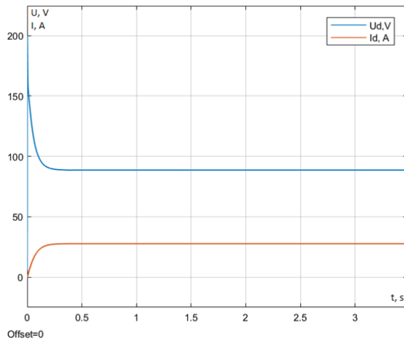
Fig. 14. The dependency of voltage u_d and current i_d of the electric arc on time under direct current
