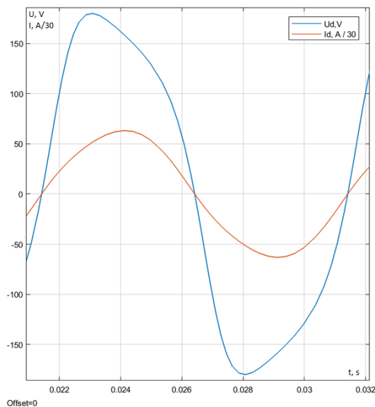
Fig. 22. The dependency of voltage u_d and current i_d of the electric arc on time, f = 100 Hz Source: compiled by the authors
