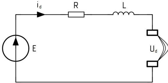
Fig. 2. The scheme of the electric arc current circuit
