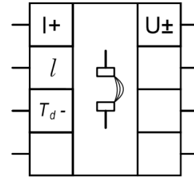
Fig. 5. The symbol for the block modeling the electric arc voltage-ampere characteristic
