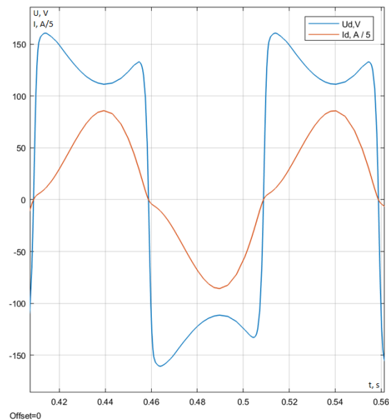
Fig. 16. The dependency of voltage u_d and current i_d of the electric arc on time, f = 10 \text{ Hz}
