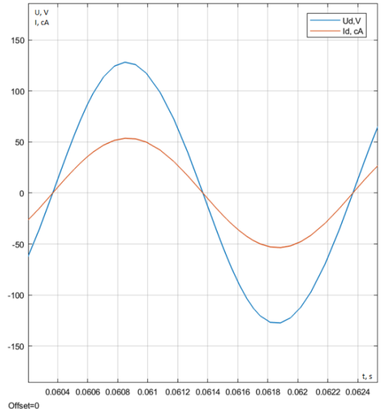
Fig. 24. The dependency of voltage u_d and current i_d of the electric arc on time, f = 500 Hz Source: compiled by the authors
