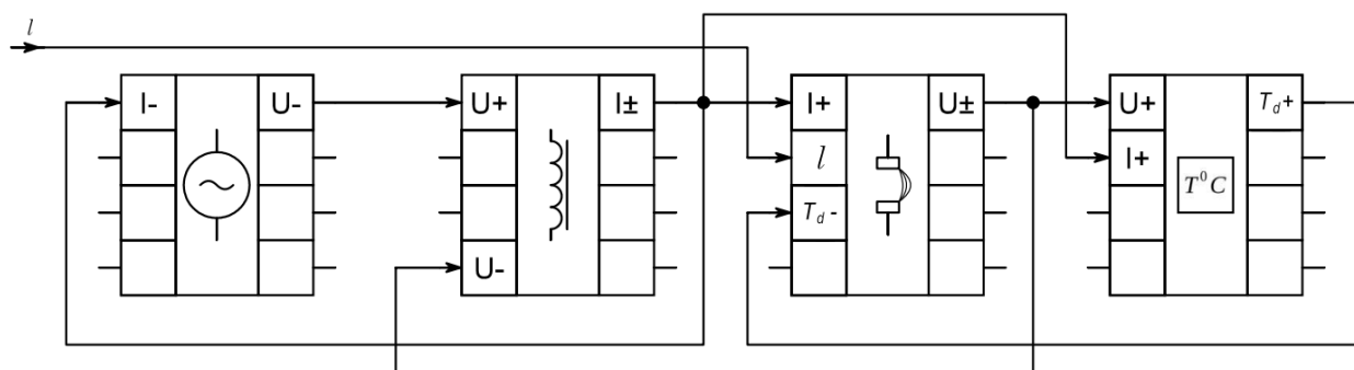
Fig. 7. The visual-block model of the electrical engineering complex with an electric arc block
