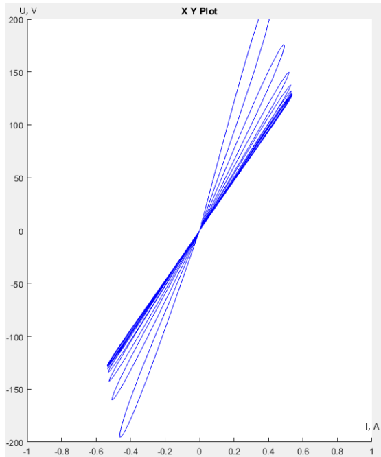
Fig. 25. The dynamic voltage-ampere characteristic (VAC) for the electric arc, f = 500 Hz
