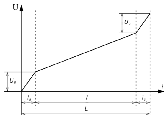
Fig. 1. Potential diagram of the arc (potential distribution with respect to the cathode)
