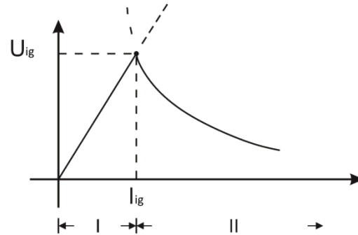
Fig. 4. Static voltage-ampere characteristic of an electric arc
