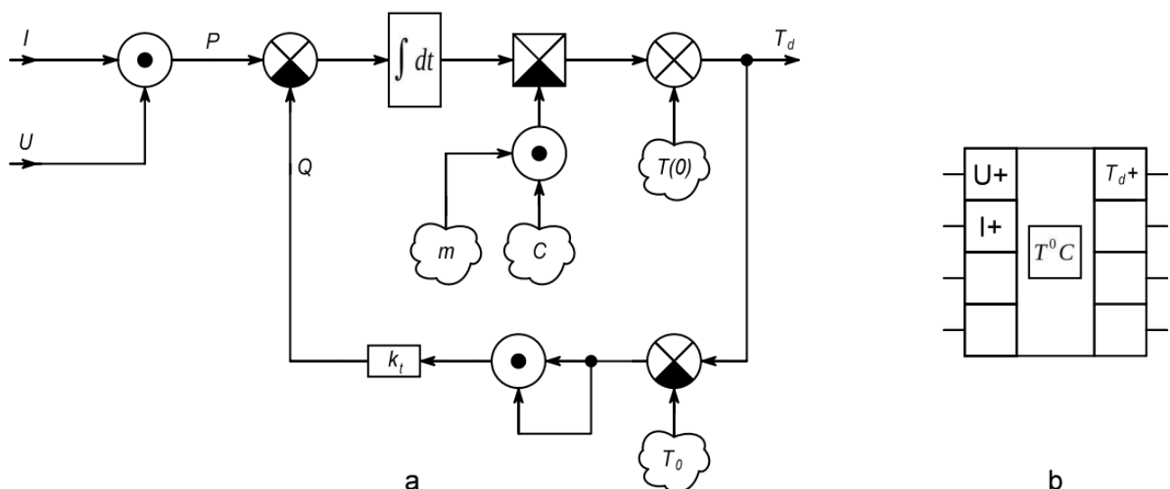
Fig. 10. Thermodynamic block: a – visual model; b – block designation
