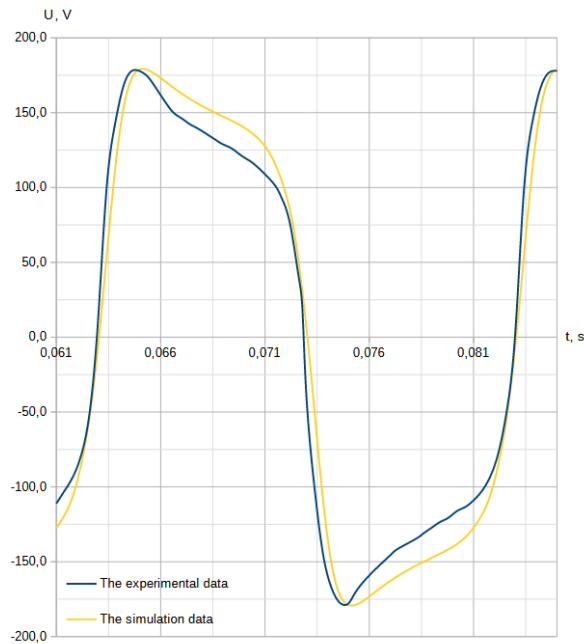
Fig. 11. The voltage dependency u_d of the electric arc over time, f = 50 Hz Source: compiled by the authors
