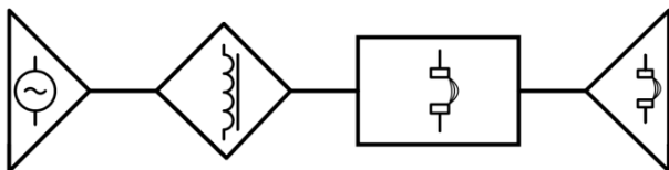
Fig. 3. The energy path diagram of the electric arc
