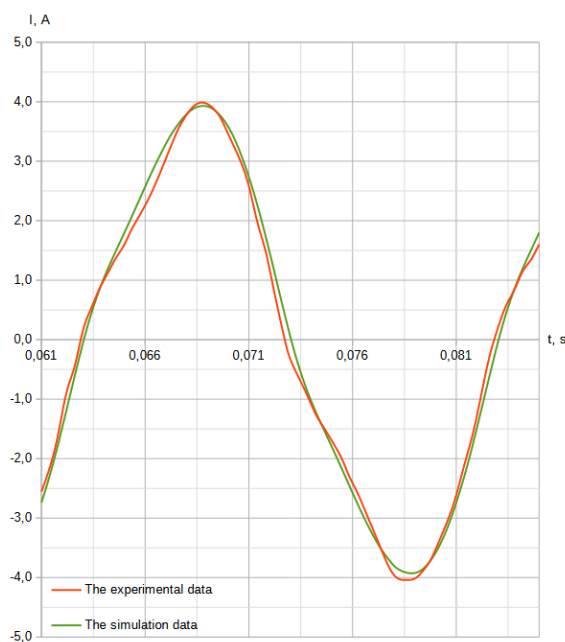
Fig. 12. The current dependency i_d of the electric arc over time, f = 50 Hz
