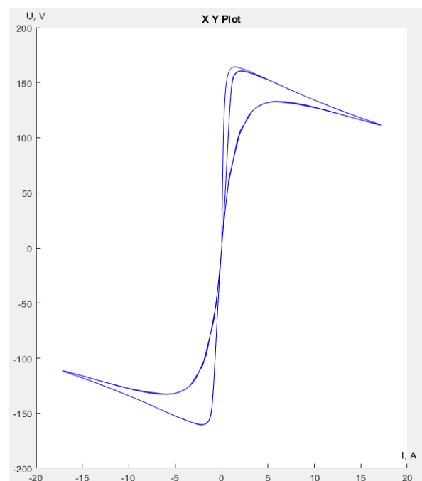
Fig. 17. The dynamic voltage-ampere characteristic for the electric arc, f = 10 \text{ Hz}
