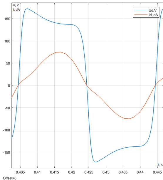
Fig. 18. The dependency of voltage u_d and current i_d of the electric arc on time, f = 25 Hz Source: compiled by the authors
