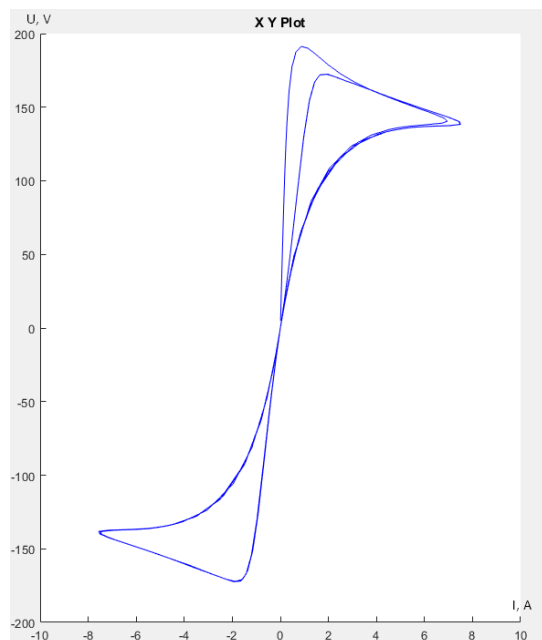
Fig. 19. The dynamic voltage-ampere characteristic of the electric arc, f = 25 Hz Source: compiled by the authors
