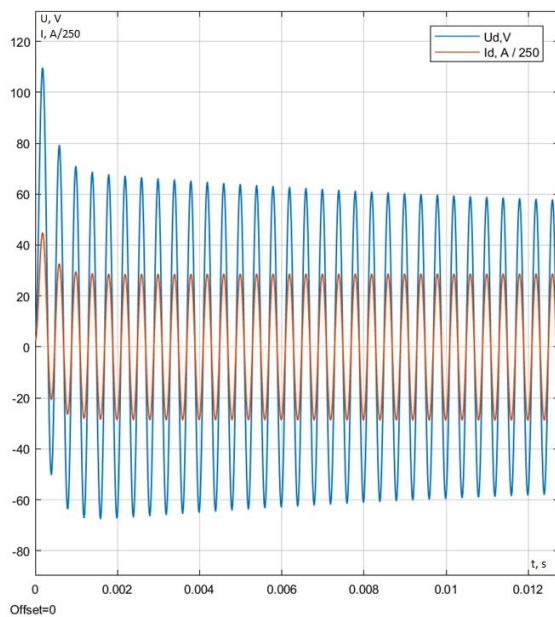
Fig. 26. The dependency of voltage u_d and current i_d of the electric arc on time, f = 2.5 kHz
