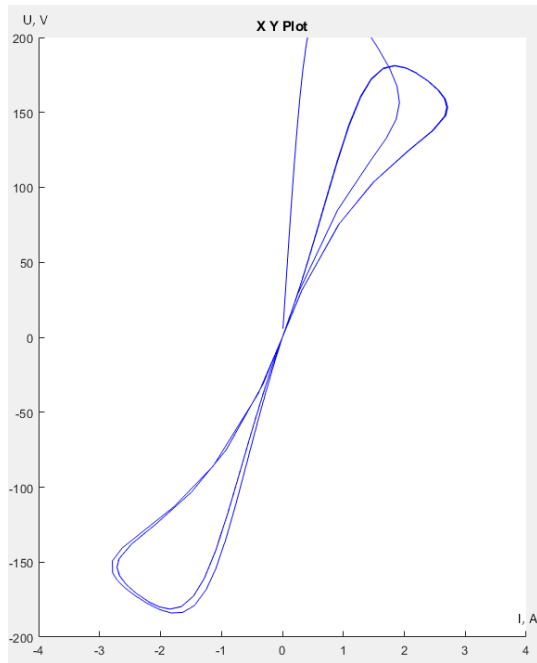
Fig. 21. The dynamic voltage-ampere characteristic of the electric arc, f = 75 Hz Source: compiled by the authors
