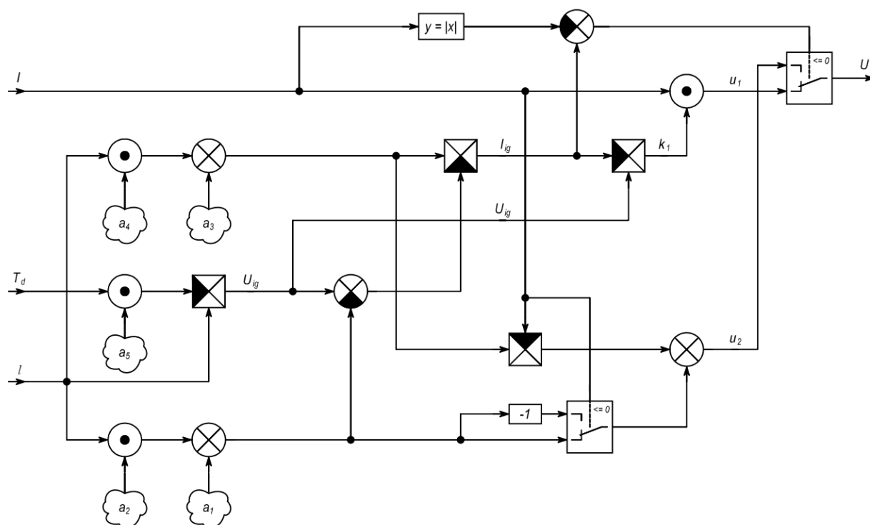
Fig. 6. The visual-block modeling of the electric arc
