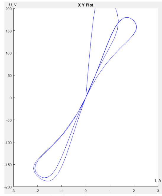
Fig. 23. The dynamic current-voltage characteristic of the electric arc, f = 100 Hz Source: compiled by the authors
